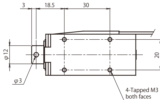
Adsorbed position
