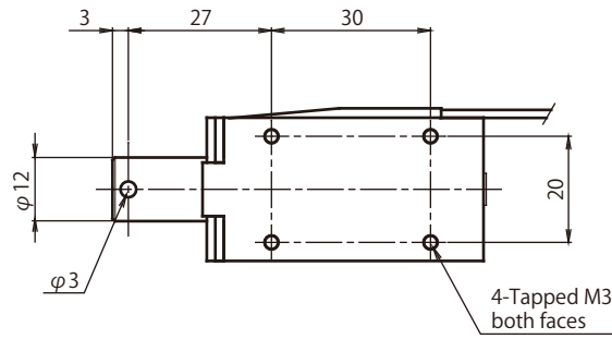
Adsorbed position
