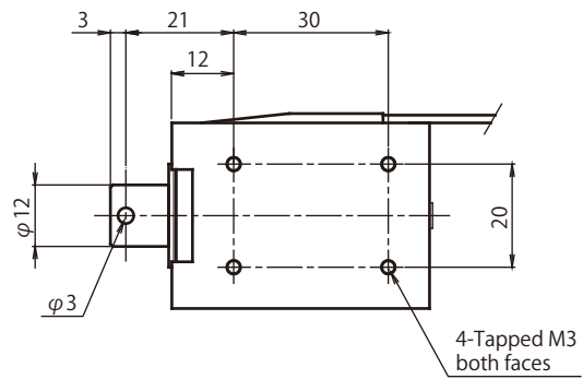
Adsorbed position
