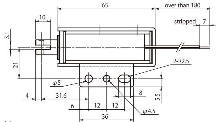
Adsorbed position
