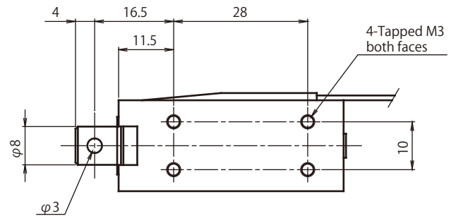
Adsorbed position
