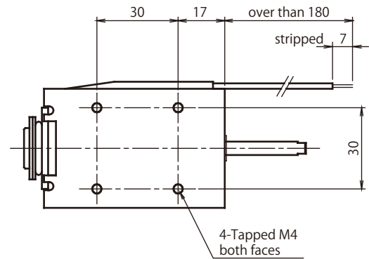
Adsorbed position
