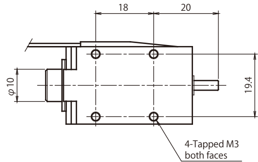
Adsorbed position
