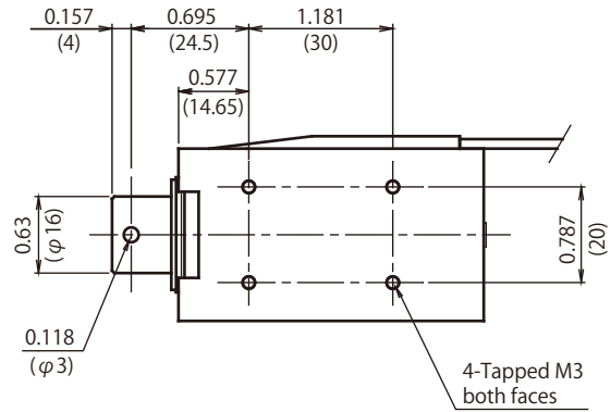
Adsorbed position
