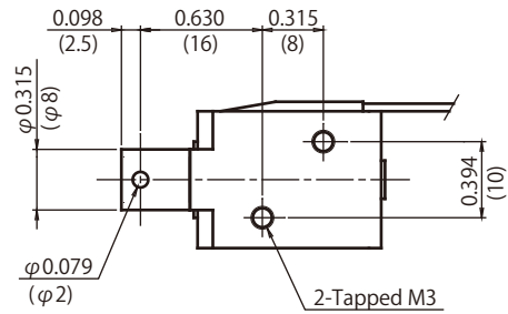
Adsorbed position
